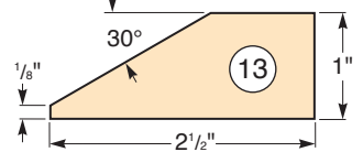
Stile (End View)
