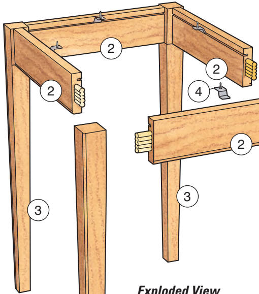
Exploded View
