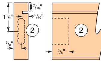
Apron (End and Inside Views)
