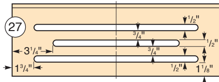
Door Frame Front Edge (Side View)
