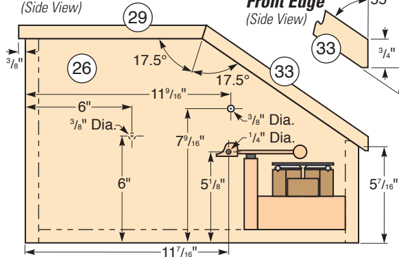
Case (Side View)
