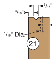
Rail (End View)
