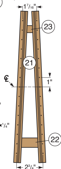
Xylophone Rack (Top View)
