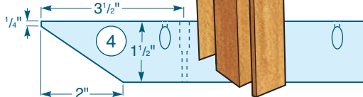
Beam (Front View)
