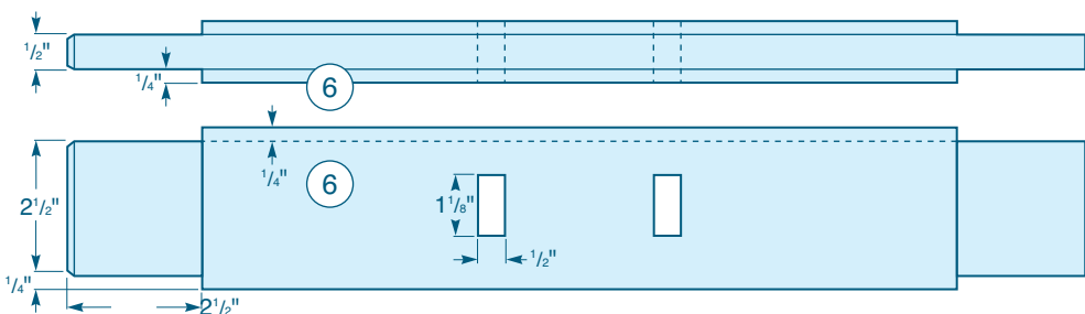
Lower Rail (Top and Front Views)
