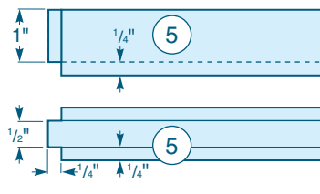
Upper Rail (Front and Bottom Views)
