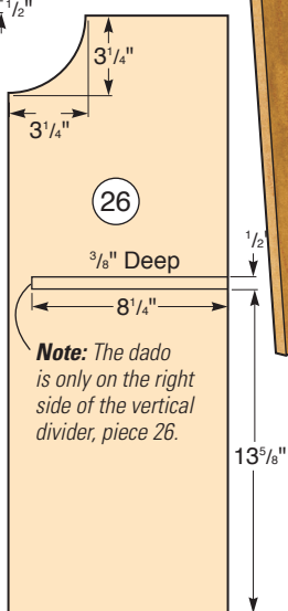
Vertical Divider (Inside View)
