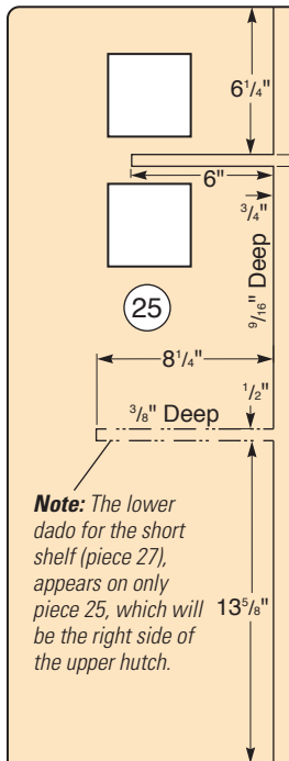
Side (Inside View)
