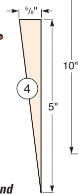
Light Wedge (Side View)
