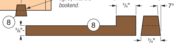
Dovetail Slides (Side and End Views)
