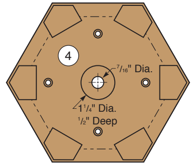
Base (Bottom and Side Views)
