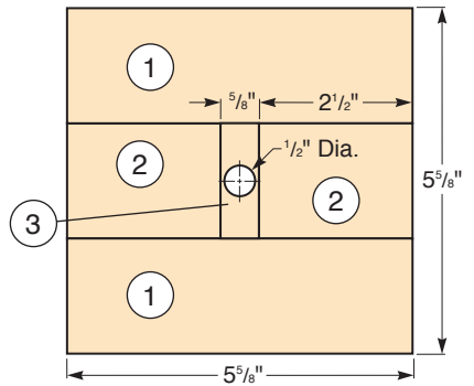
Base (Bottom and Side Views)
