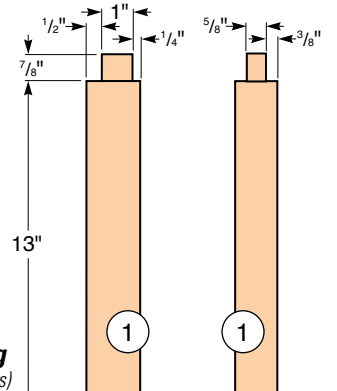
Headboard Leg (Front and Side Views)
