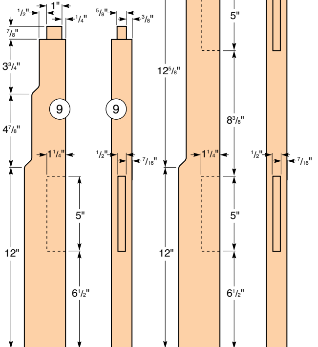
Footboard Leg (Front and Side Views)
