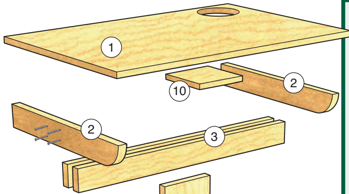
Exploded View
